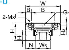
MGN5HL-0
