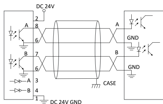
ST-A signal translator
