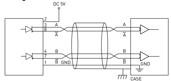
ST-A signal translator
