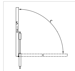
In this position, the point of gravity S is close to or directly on the pivot point. A weak spring force is required. Both strokes are fully extended.
